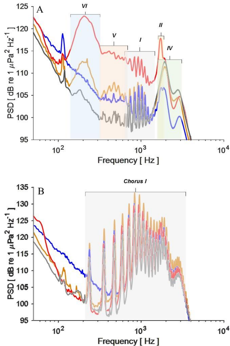
Figure 7. Power spectrum of averaged RMS emphasizing the frequency (log) components that occurs continually in the recordings during A. night (between ~17:30 to 00:00 h) and B. after midnight (between ~00:00 to 05:00 h), showing different peaks of fish chorus dominant frequency in MLPZ 3 (blue line), MLPZ 4 (red line), PGA 1 (grey line) and PGA 2 (orange line).
