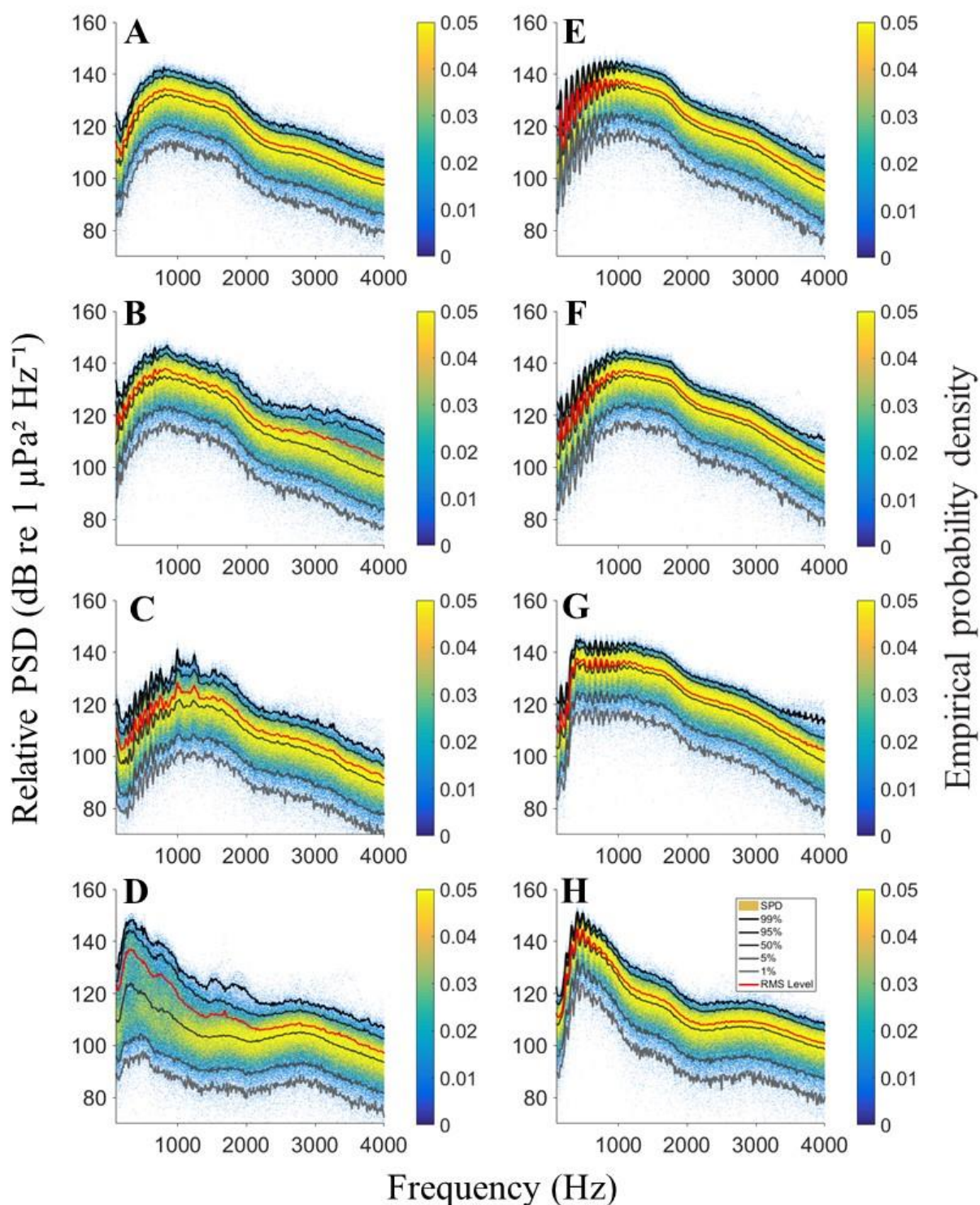
Figure 29. Power spectra of continuous sounds from rivers confluences. A) Negro, B. Machado, C. Pakaas, D. Soterio, E. Guapore, F. Cautario, G. Machupe and H. Branco. Low and high frequency limits of 100- 4000. Hann windows type, window length 0.1s and overlap of 50%.
