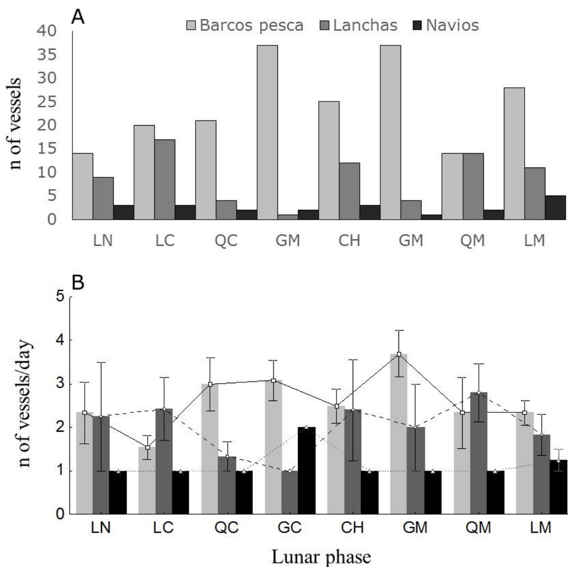
Figure 22. Number of fishing vessels A. total and B. per day (indicating mean \pm standard error), detected in the different phases of the moon.
