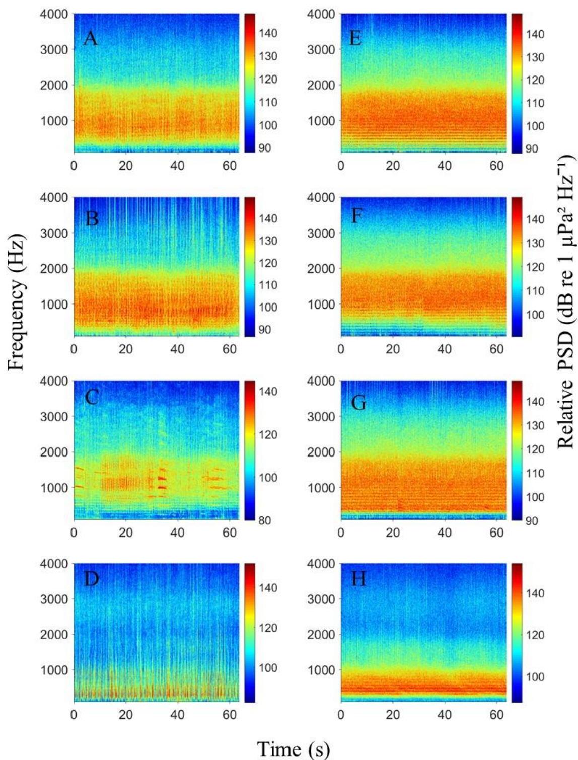
Figure 28. Sonograms of underwater recordings from various rivers: A) Negro; B) Machado; C) Pakaas; D) Soterio, E. Guapore, F) Cautario; G) Machupe and H) Branco. Low and high frequency limits of 100- 4000 Hz, Hann window, window length 0.1s.
