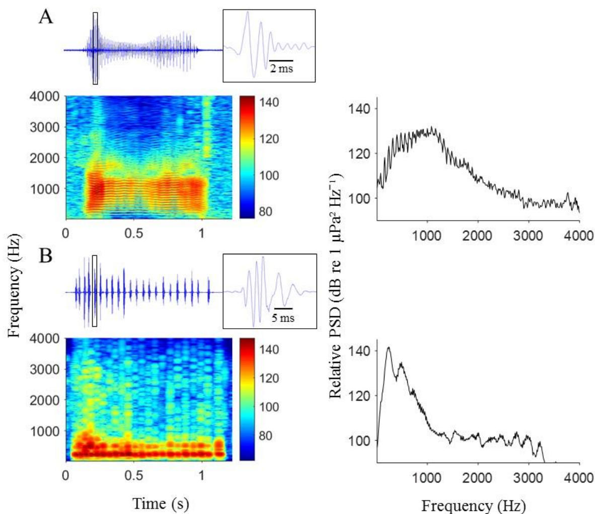
Figure 26. Prochilodontidae disturbance calls spectrograms, waveforms (individual pulse indicated by squares). A) S. insignis and B) P. nigricans . Hann windows type, DFT size 512 and overlap of 98.8%. Low and high frequency limits of 100- 4000 Hz. Hann windows type, window length 0.1s.
