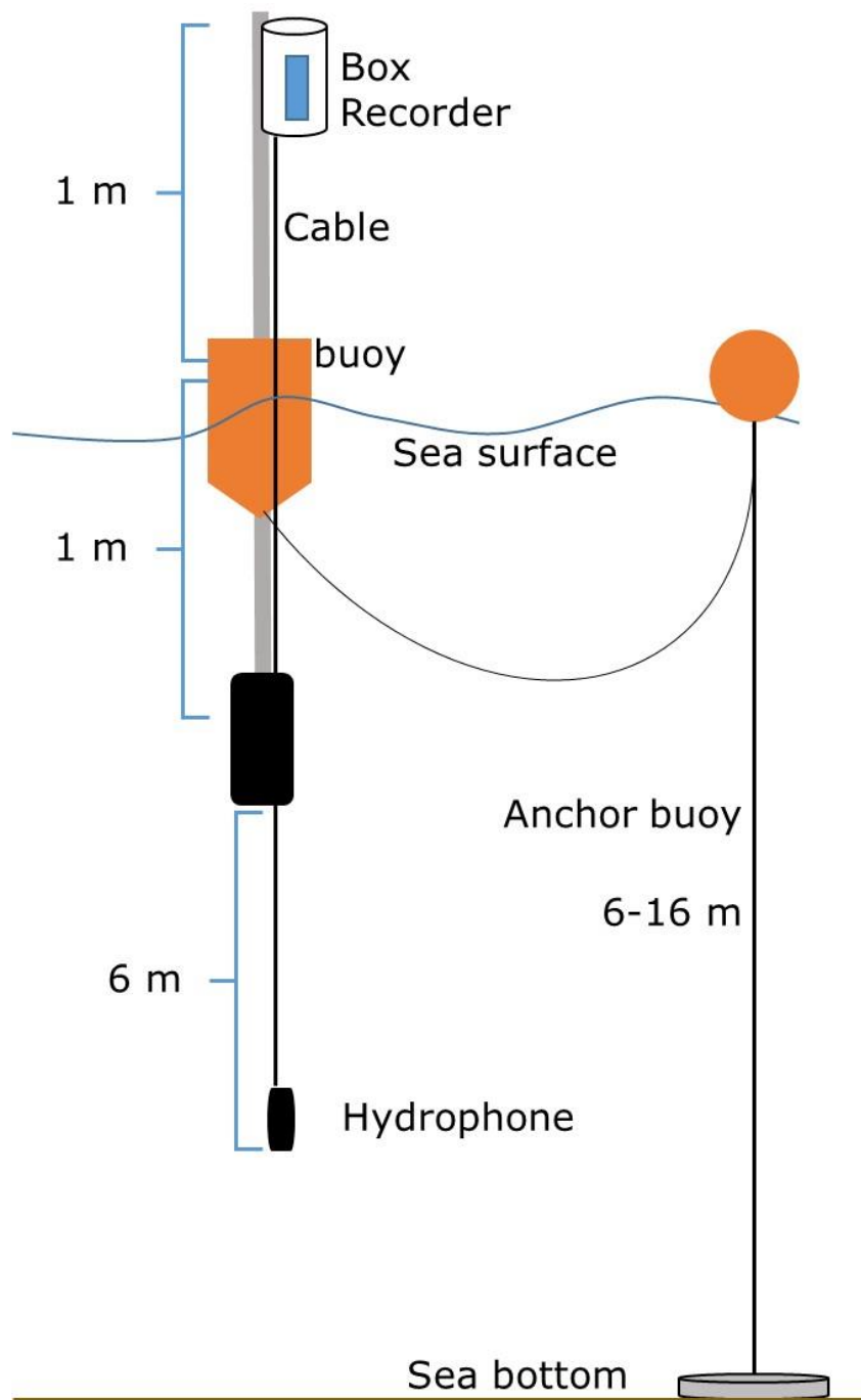
Figure 2. Sonobuoy configuration deployed in Tamandaré and Porto de Galinhas
