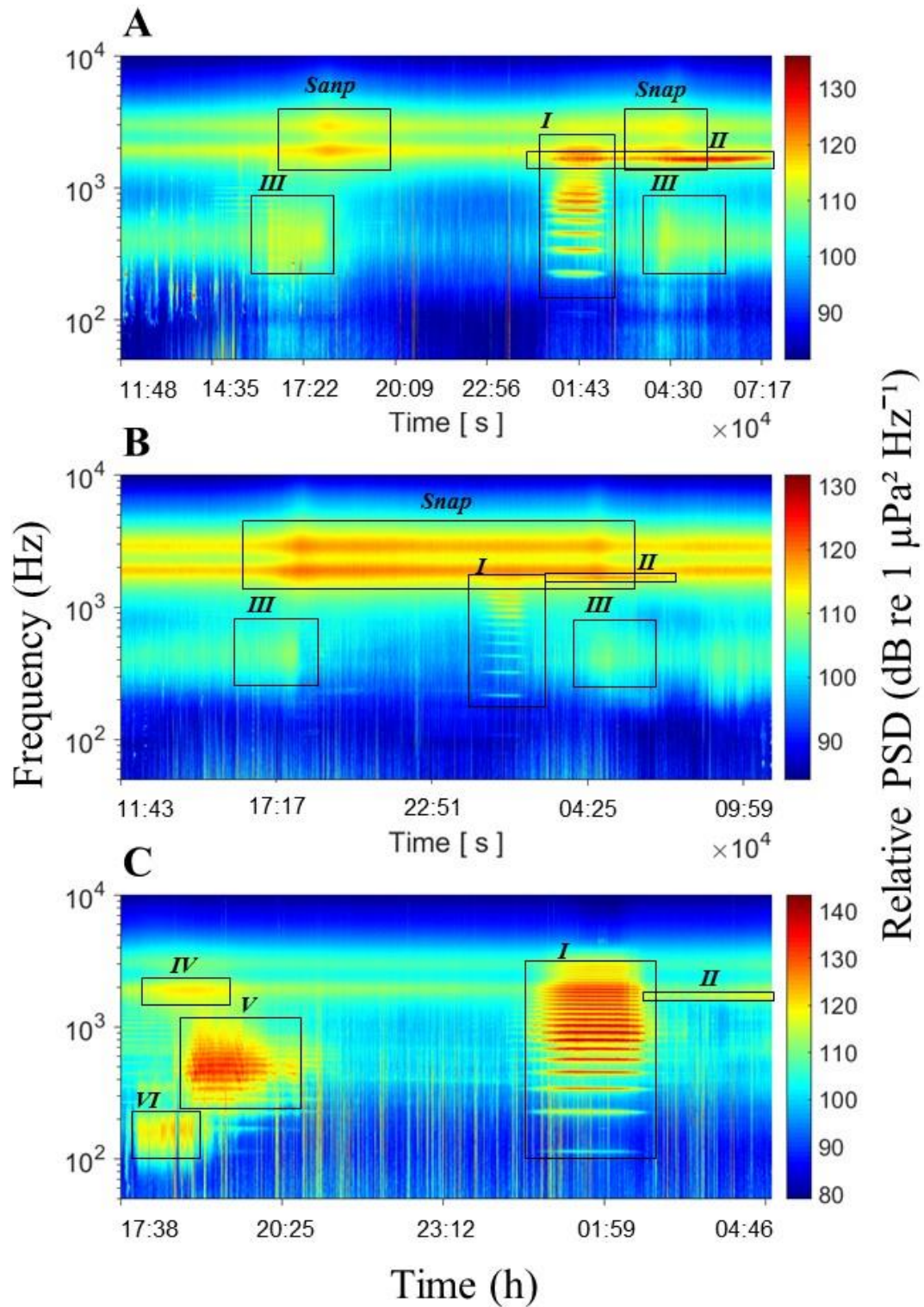
Figure 3. Spectrograms (sonograms) showing the time variation of the frequency and the power spectral density (PSD) of recording near to “Ilha da barra” reef in Tamandaré. A. MLPZ 1 (Jan, 24); B. MLPZ 2 (Jan, 26) and C. MLPZ 3 (Feb, 04), highlighting the main acoustics signals. “Snap” corresponding to crustacean sounds and “Chorus I”, “Chorus II”, “Chorus III”, “Chorus IV”, “Chorus V” and “Chorus VI” considered as fish sounds.
