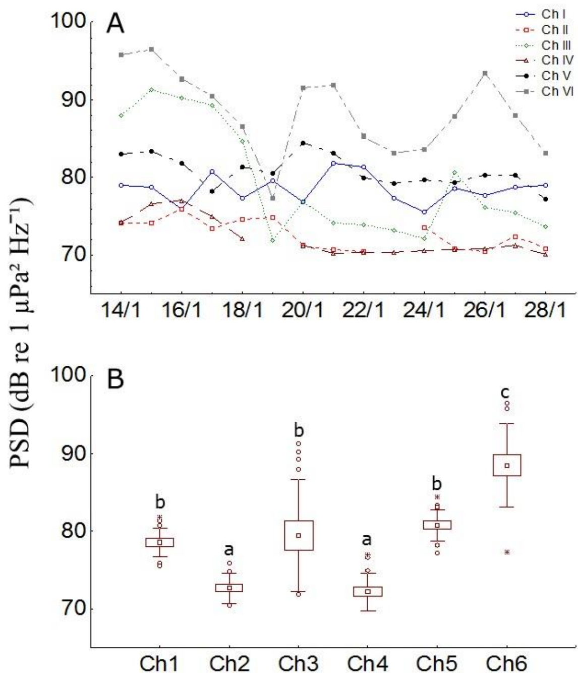
Figure 15. Daily energy pattern (dB re 1 \mu\text{Pa}^2 \text{Hz}^{-1} ) of fish choirs detected three days after the full moon in the Marine Life Preservation Zone of Tamandaré during the summer. Different letters indicate significance difference ( p < 0.05 ).
