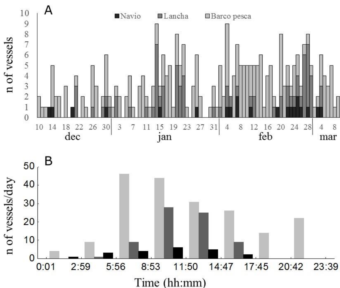
Figure 21. A. Number of vessels per day and B. standard of schedules of the total number of vessels detected.
