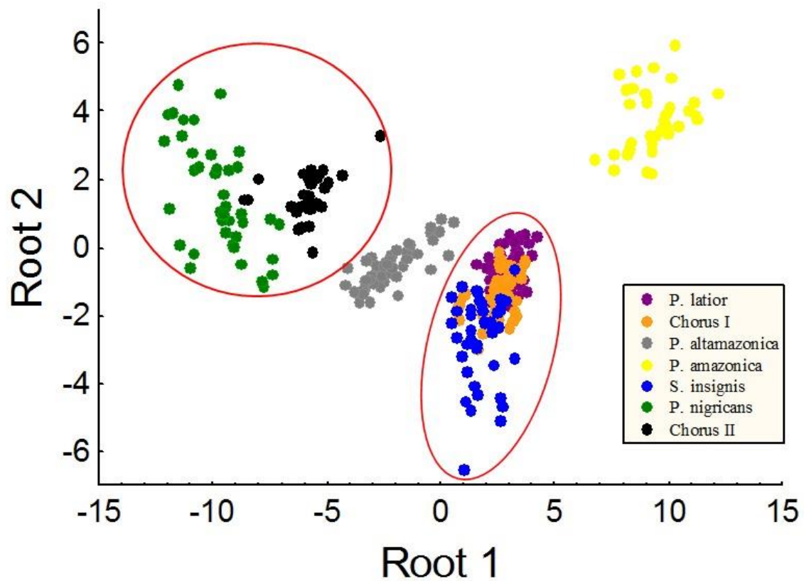
Figure 32. Canonical discriminant scores generated by the first two discriminant functions to illustrate the separation of different Amazon fish using acoustic parameters. Based on a total of 8 discriminant functions, with the factor 1 and 2 was 69.7%.
