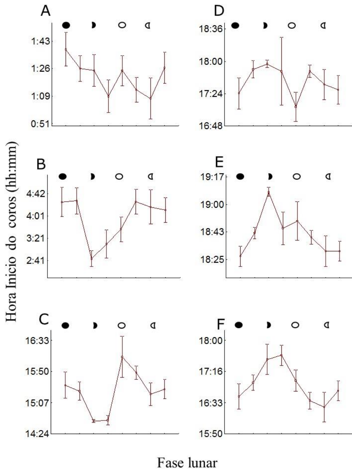
Figure 17. Patterns of Fish Chorus initial times in the different lunar cycle phase. A. Chorus I; B. Chorus II; C. Chorus III; D. Chorus IV; E. Chorus V and F. Chorus VI.
