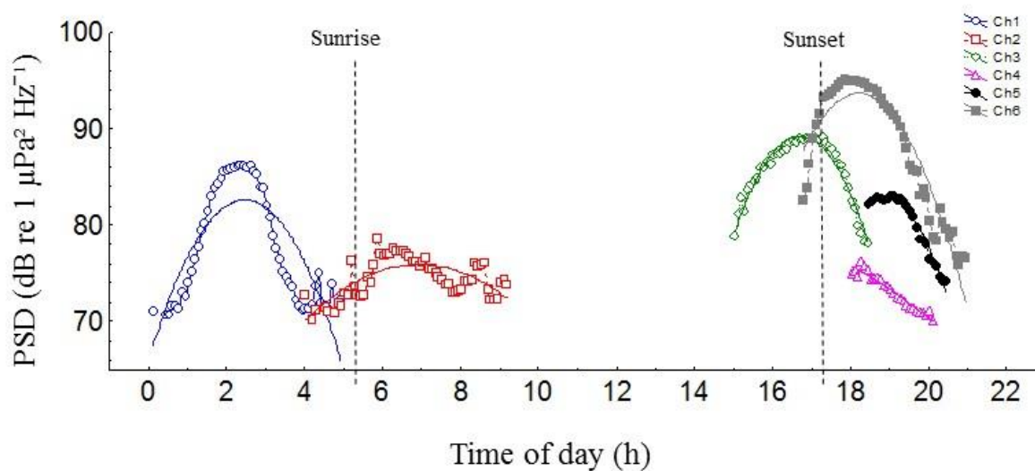
Figure 14. Daily pattern distribution of fish chorus related to the acoustic energy (dB re 1 \mu\text{Pa}^2 \text{ Hz}^{-1} ) detected in the Marine Life Preservation Zone of Tamandaré during the summer. Dotted lines indicate local time at sunrise (5:15) and sunset (5:30 pm).
