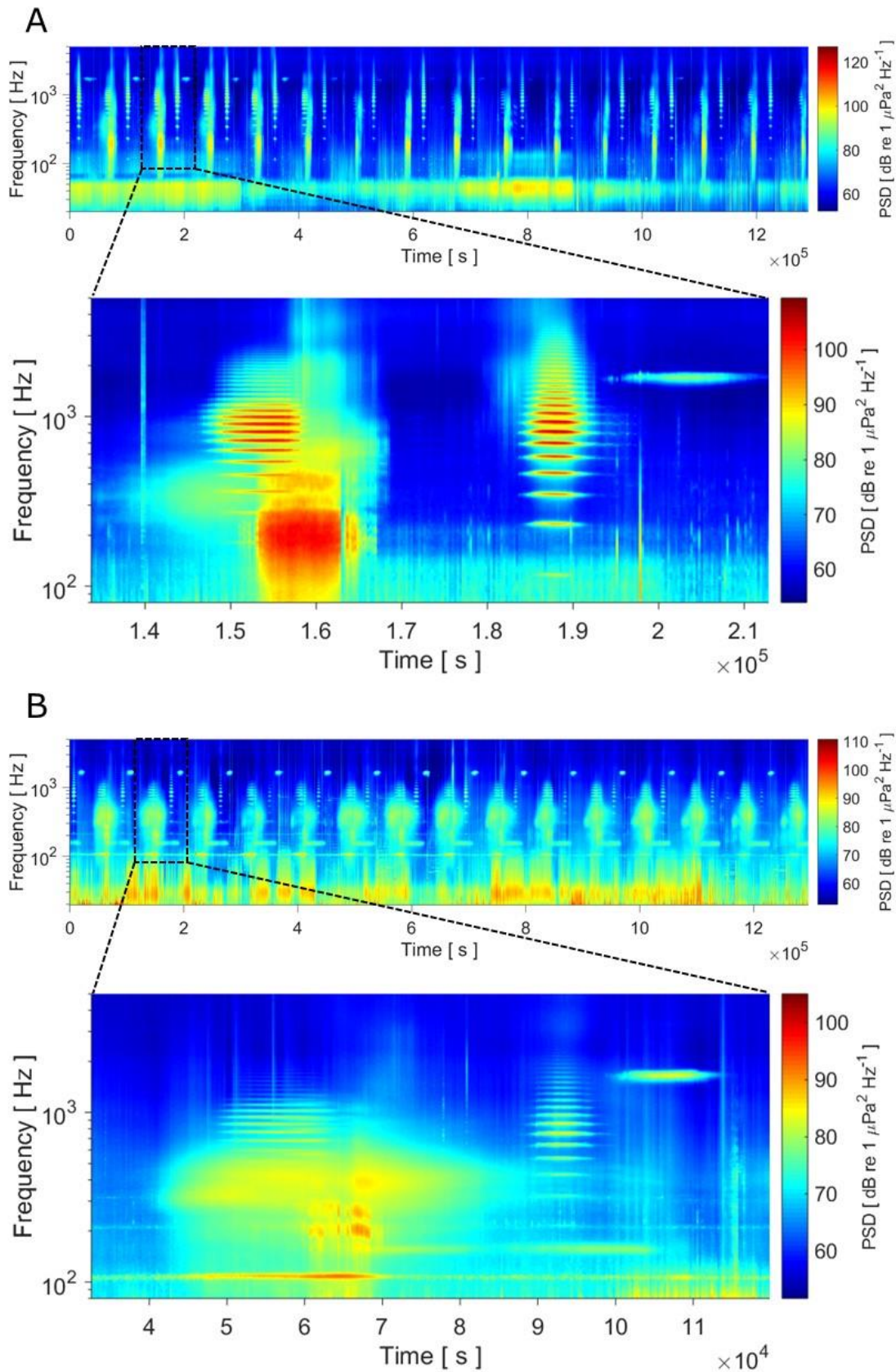
Figure 18. Spectrograms of 15 days after full moon in A. February, (summer) and B. June, 12-27 (winter). The spectrograms were produce using 1024 point Hanning window (50% overlap), plotted on a logarithmic frequency scale between 80 and 5000 Hz.
