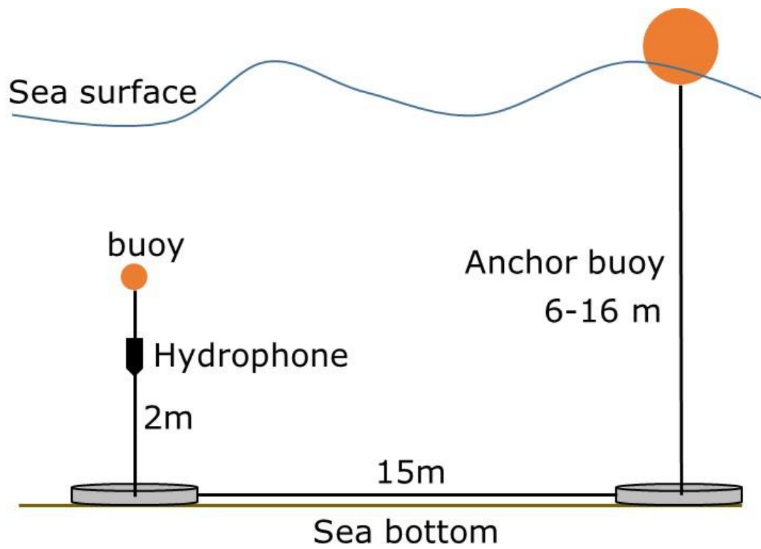
Figure 12. Autonomous acoustic underwater recorder configuration module.
