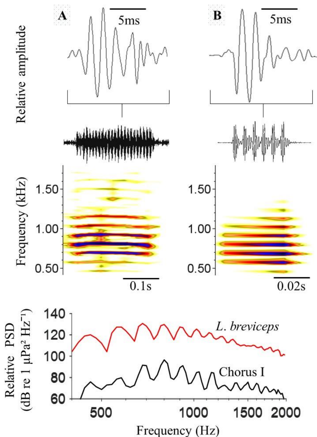
Figure 10. Individual call waveform, spectrogram and power spectrum of A. Chorus I and B. Larimus breviceps sound file recorder under stress by Fish and Mowbray 1970, available in http://www.fishbase.org/physiology/FishSoundsSummary.php?autoctr=149 .
