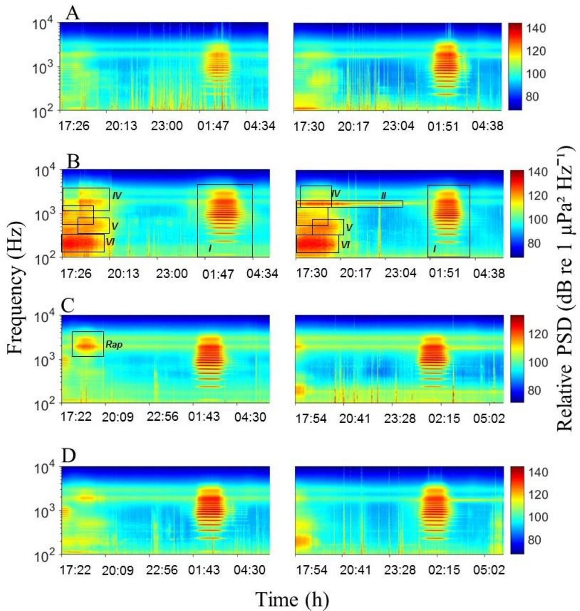
Figure 5. Spectrograms showing the time variation of the frequency and the power spectral density (PSD) of recordings between ~17:30 to 05:30 in Tamandaré and Porto de Galinhas in March. A. MLPZ 3; B. MLPZ 4; C. PGA 1 and D. PGA 2, highlighting the mainly acoustics signals. “Chorus I”, “Chorus II”, “Chorus IV”, “Chorus V” and “Chorus VI” were considered as fish sounds (overlapping during the sunset), and “Rap” corresponds to crustacean sounds.
