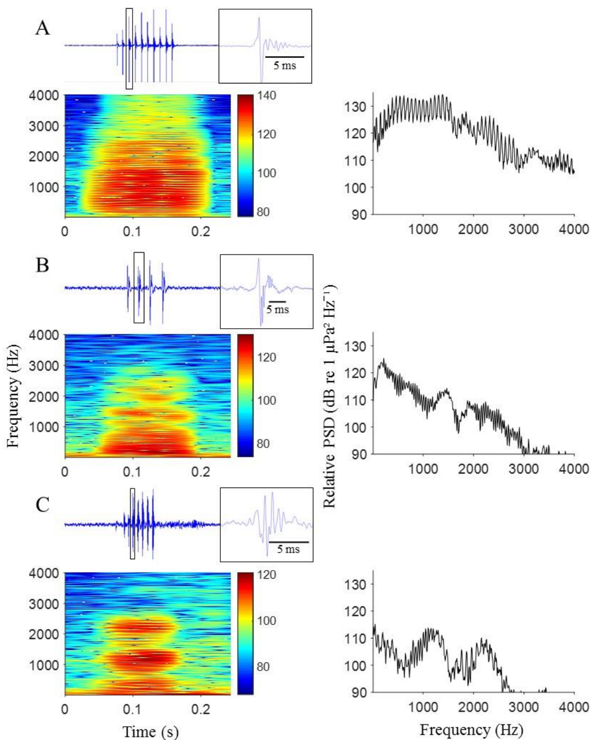
Figure 25. Curimatidae disturbance calls spectrograms, waveforms (individual pulse indicated by squares) and spectrum of A) P. latior ; B) P. altamazonica ; C) P. amazonica . Hann windows type, DFT size 512 and overlap of 98.8%. Low and high frequency limits of 100- 4000 Hz. Hann windows type, window length 0.1s.
