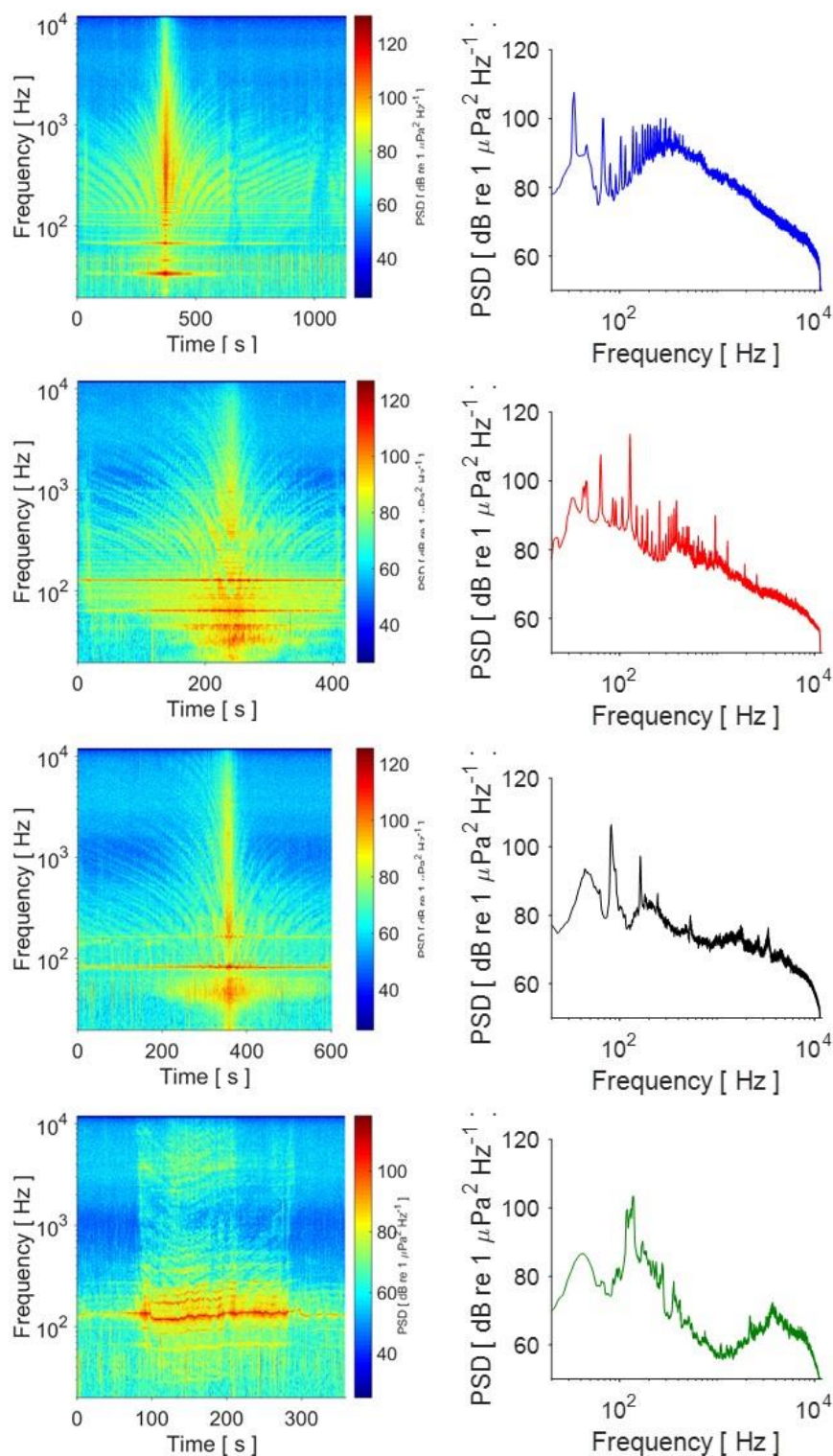
Figure 20. Spectrogram and power spectrum A. fishery vessel B. recreational boats. The spectrograms were produce using 1024 point Hanning window (99.9% overlap), plotted on a logarithmic frequency scale between 20 and 10000 Hz.
