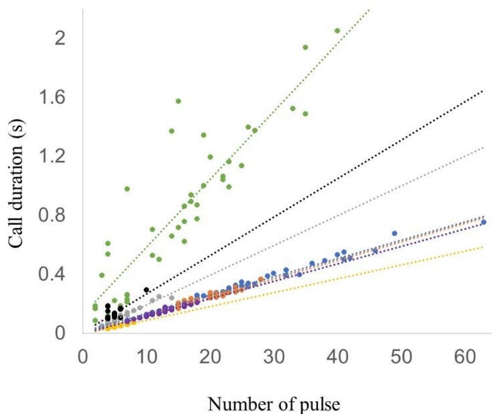
Figure 30. Positive relationship of call duration and number of pulse in disturbance and voluntary calls detected in the Madeira basin
