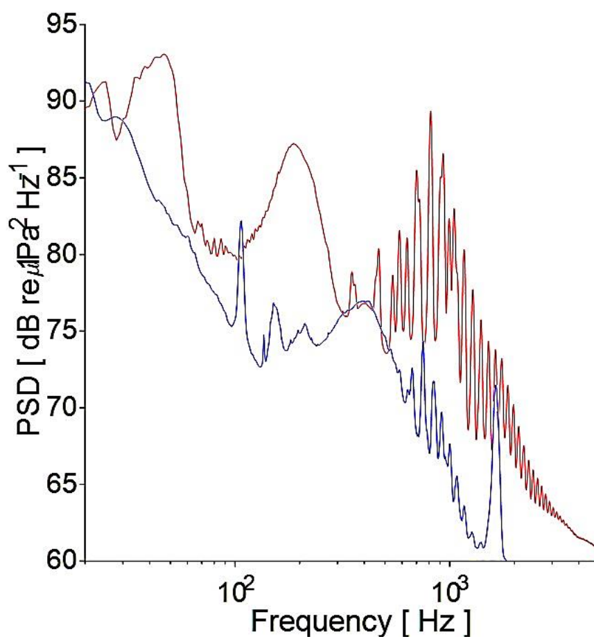
Figure 19. Spectrum of 15 days after full moon in February (red line) and B. June, 12-27 (blue line), plotted on a logarithmic frequency scale between 20 and 5000 Hz
