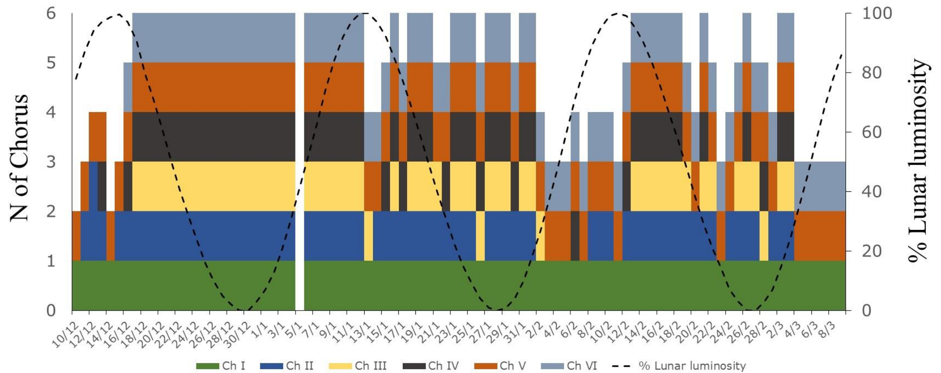
Figure 13. Daily patterns of different fish chorus detected in the Marine Life Protection Zone in Tamandaré during the summer. % of lunar luminosity (dotted dash line).
