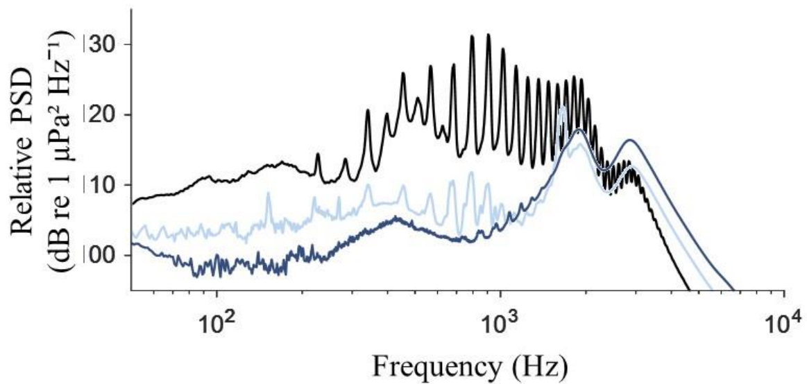
Figure 4. Average power spectrum (spectra) averaged emphasizing the frequency (log) components that occur continually in the recordings around the “Ilha da barra” reef. MLPZ 1 Jan, 24 (grey line), MLPZ 2 Jan, 26 (blue line) and C MLPZ 3 Feb, 04 at night (black line). The peaks of dominant frequency correspond to “Chorus II” (~1700 Hz, grey line), “Chorus IV” (~1800 Hz, blue line) and “Chorus I” (~900 Hz, black line), with broad frequency band masking the other signals.
