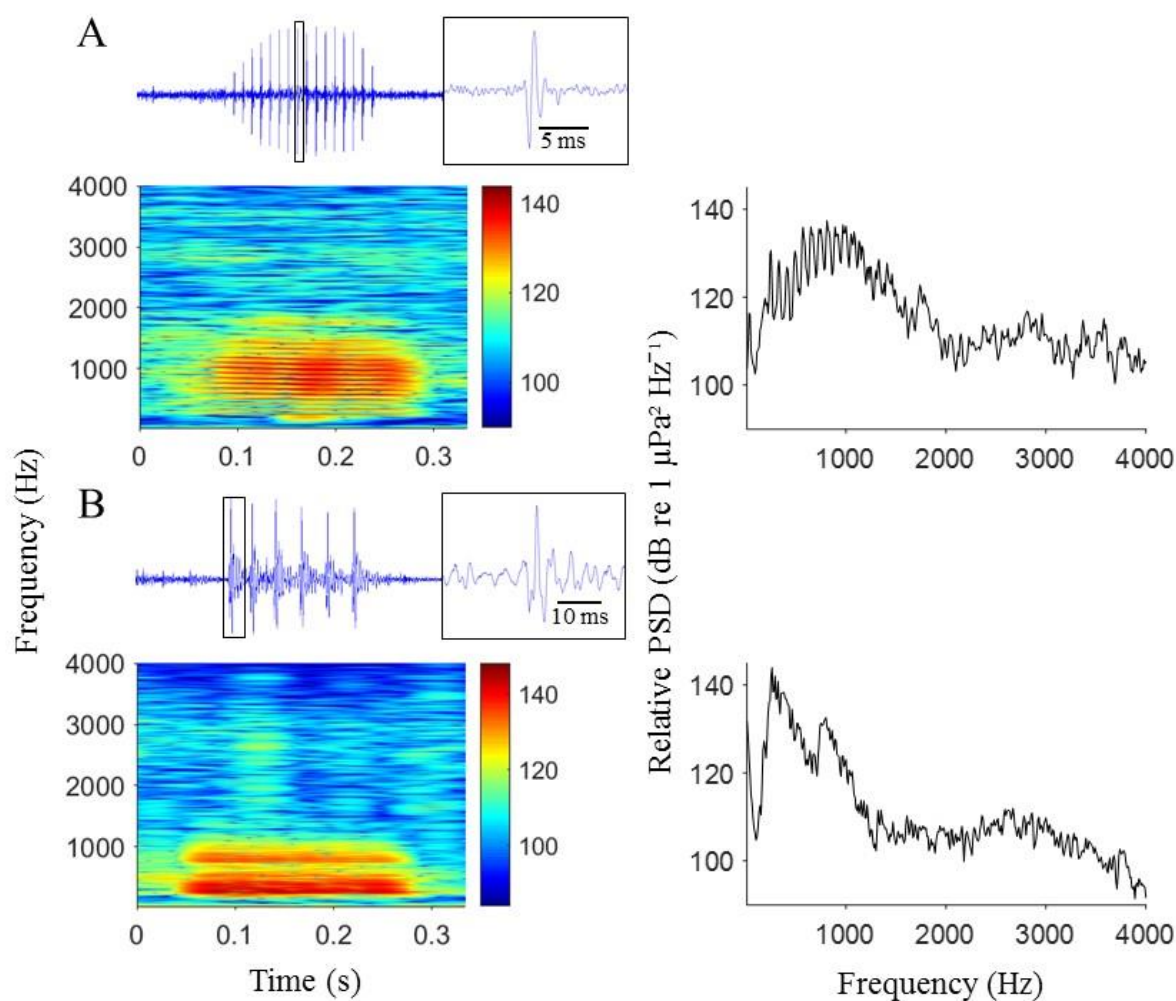
Figure 27. Underwater voluntary calls spectrograms, waveforms (individual pulse indicated by squares). A) Chorus 1 and B) Chorus II. Hann windows type, DFT size 512 and overlap of 98.8%. Low and high frequency limits of 100- 4000 Hz. Hann windows type, window length 0.1s.
