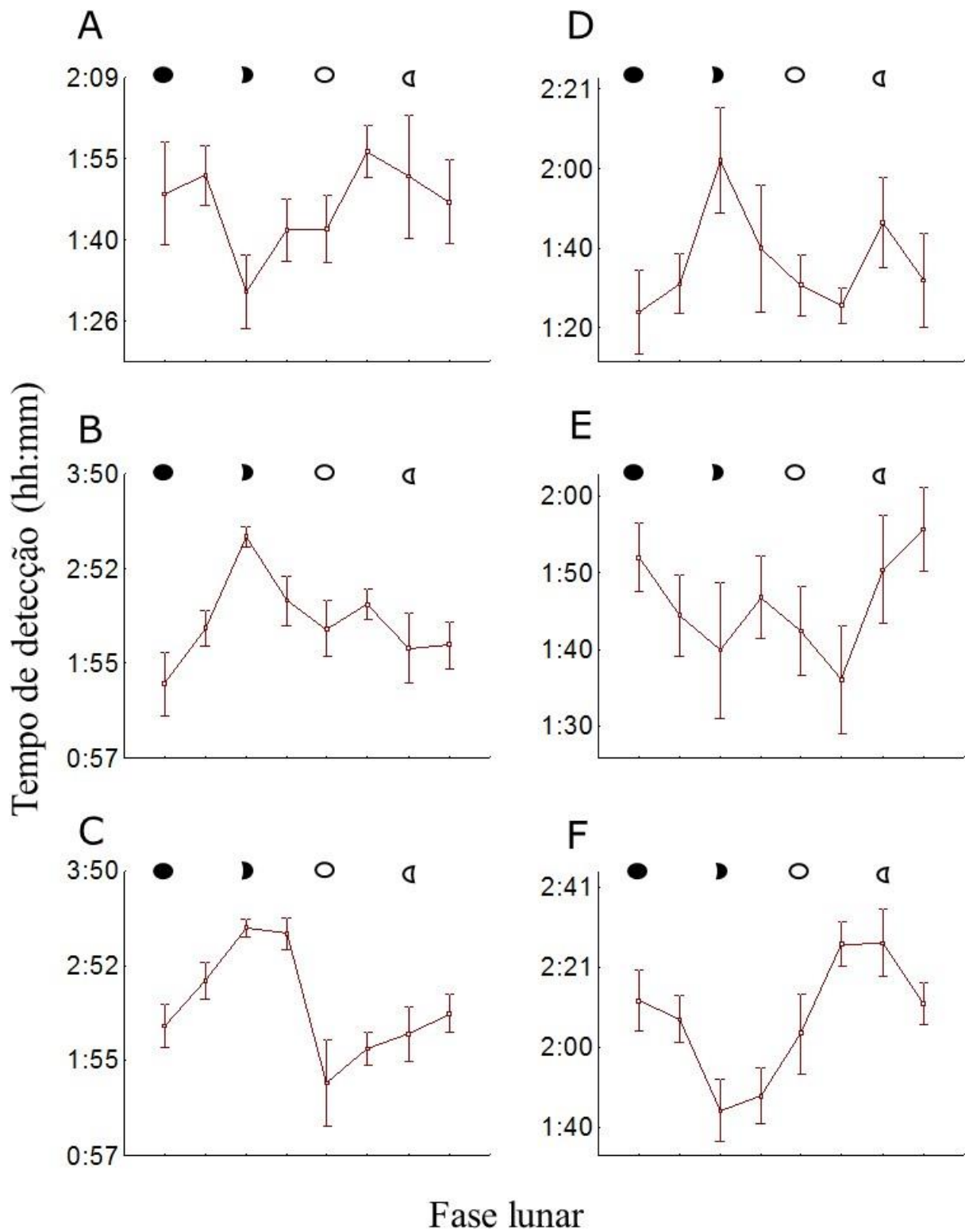
Figure 16. Patterns of total detection time of fish chorus in the different lunar phase. A. Chorus I; B. Chorus II; C. Chorus III; D. Chorus IV; E. Chorus V and F. Chorus VI.
