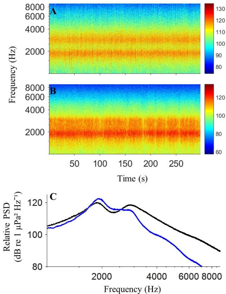
Figure 6. Spectrograms of crustacean sounds A. “Snap” and B. “Rap” (recorded in Porto de Galinhas) and C. power spectrum of “Snap” (black line) and “Rap” (blue line) frequency.
