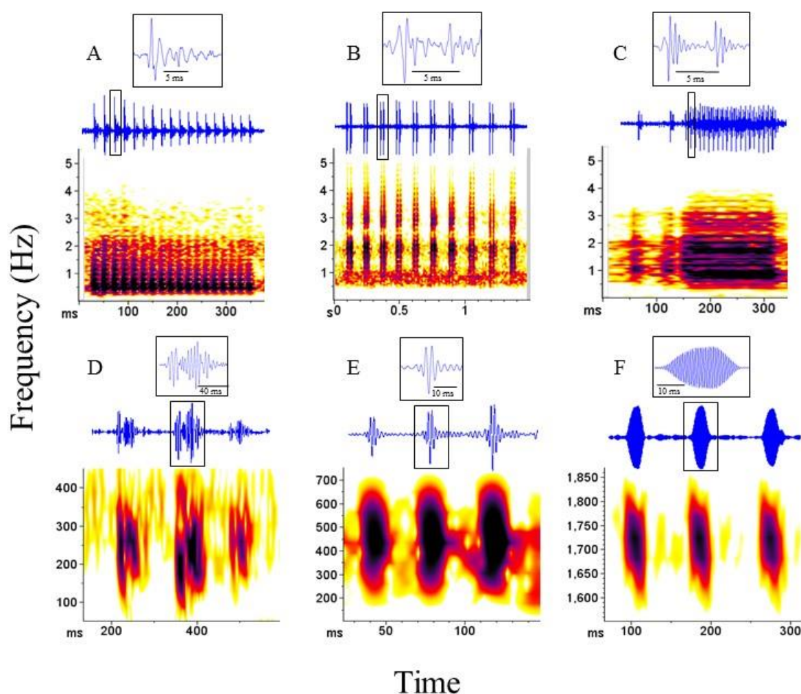
Figure 9. Oscillograms (waveforms), spectrograms of individual calls (below) and respective pulse magnified (quadrants), presenting a train of pulses in A. "Chorus V", B. "Chorus IV" (paired), C. "Chorus I" (paired), D. "Chorus VI", E. "Chorus III" and F. "Chorus II".
