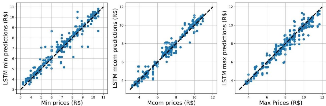
Figure 7 - Scatter Plot of the Real Minimum (Min), Maximum (Max) and Most Common (Mcom) Prices Against the LSTM Forecast for Each Variable
