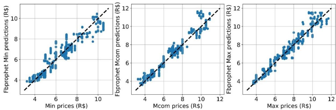
Figure 6 - Scatter Plot of the Real Minimum (Min), Maximum (Max) and Most Common (Mcom) Prices Against the Fbprophet Forecast for Each Variable
