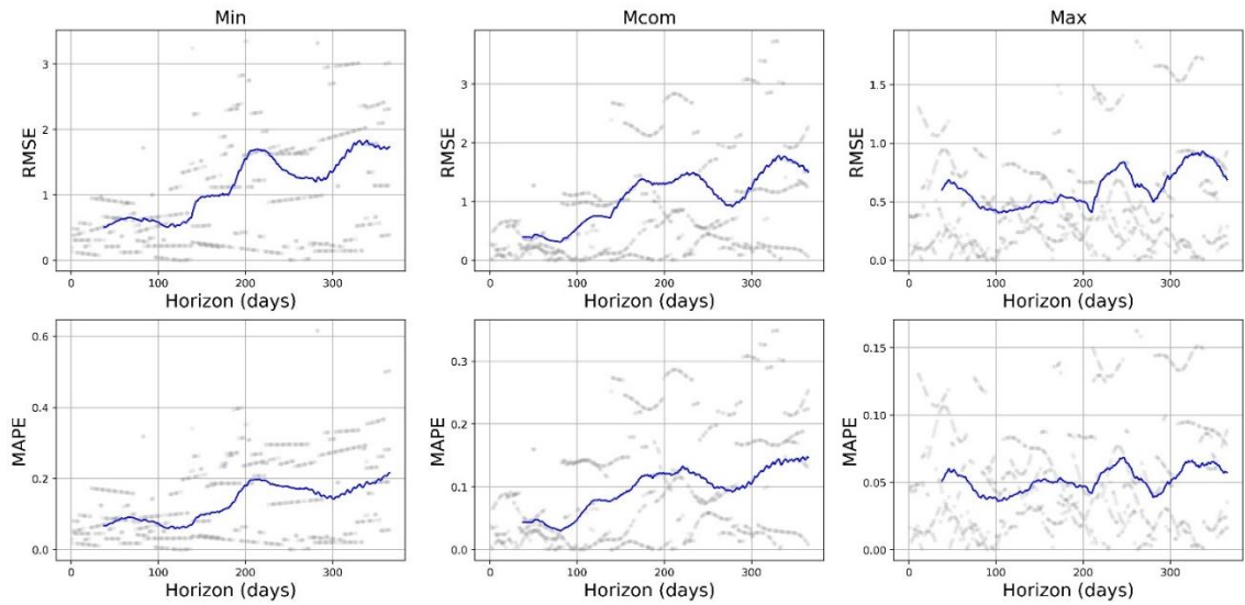
Figure 5 - Variation of Root Mean Square Error (RMSE) and Mean Absolute Percentage Error (MAPE) of the FbProphet Models in the Price Variables in Different Time-Horizons of Forecasting. Grey points are the error metric for each day and the blue line is the moving average of the error metric in the cross-validation process
