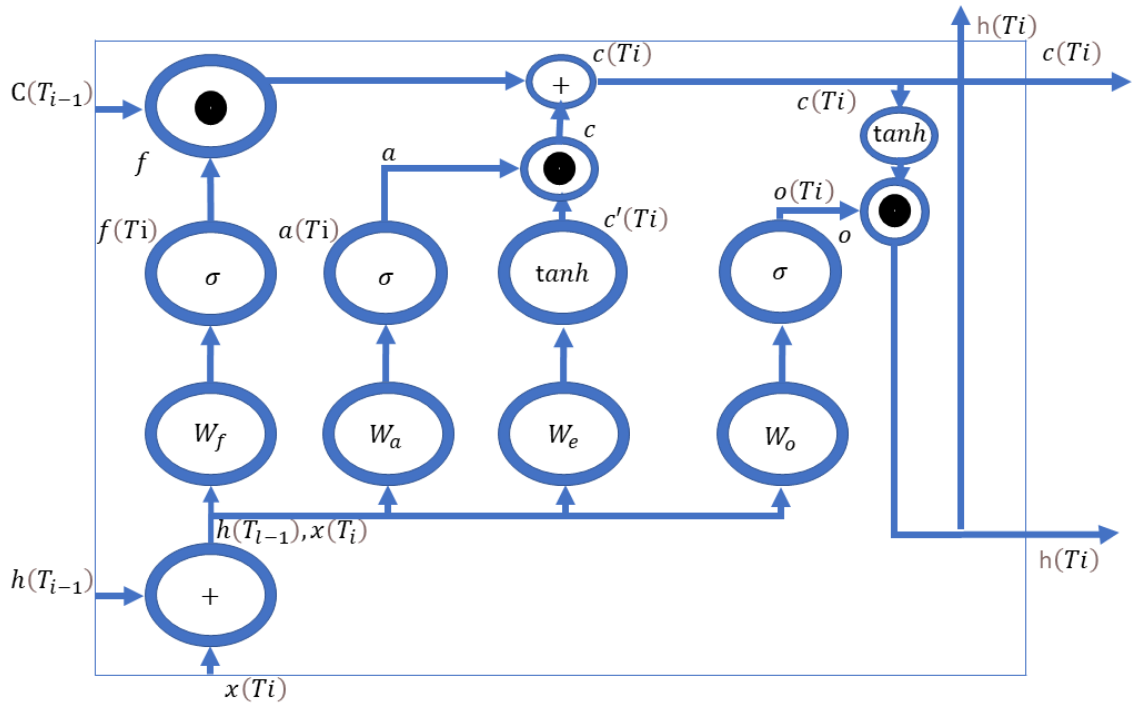
Figure 1 - The LSTM Layer Structure (adapted from Greff et al., 2017)
